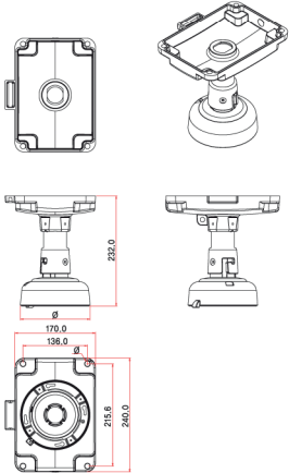
Ceiling Mount Bracket 5012-0423
