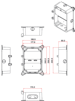
Junction Box 5012-0460
