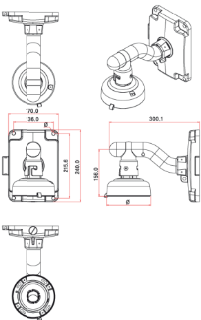
Wall Mount Bracket 5012-0412
