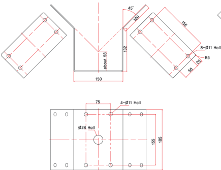
Corner Mount Adaptor 5012-0433
