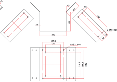
Pole Mount Adaptor 5012-0434
