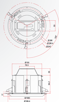
Flush Mount Bracket 5012-0418
