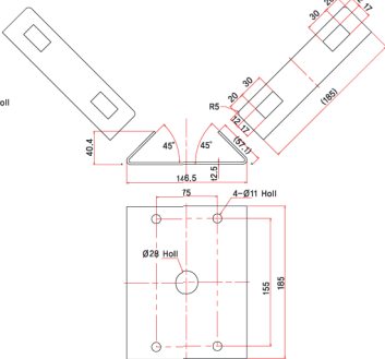
Pole Mount Adaptor 5012-0434
