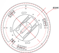
Hard Ceiling Mount Bracket 5012-0426
