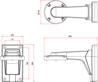
Wall Mount Bracket 5012-0413
